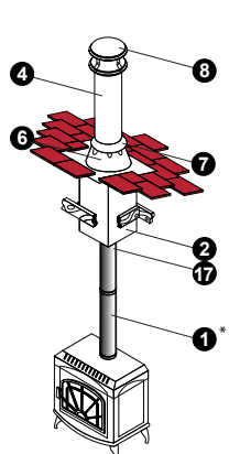
Manufactured Home *DVL stovepipe required for this installation
