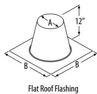
Flat Roof Flashing
