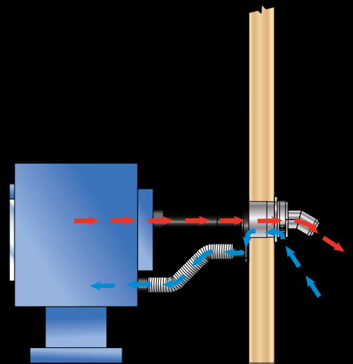
Horizontal Installations
