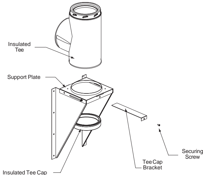
FIGURE 15 - Explosion View - Wall Support, Insulated Tee and Tee Cap, Tee Cap Bracket and securing Screw.
