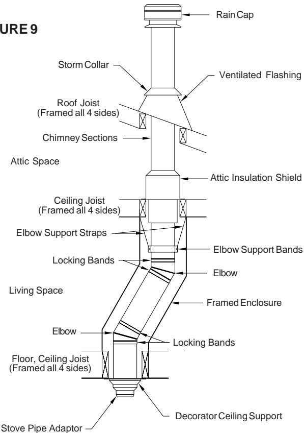
Offset (Elbow) Installation
