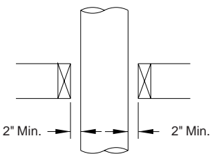
FIGURE 2 Typical Joist Framing
