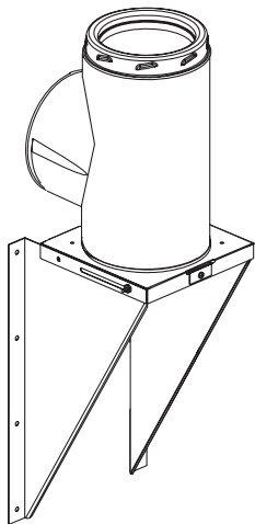
FIGURE 16 - Assembled Wall Support with Tee Cap Secured in Place
